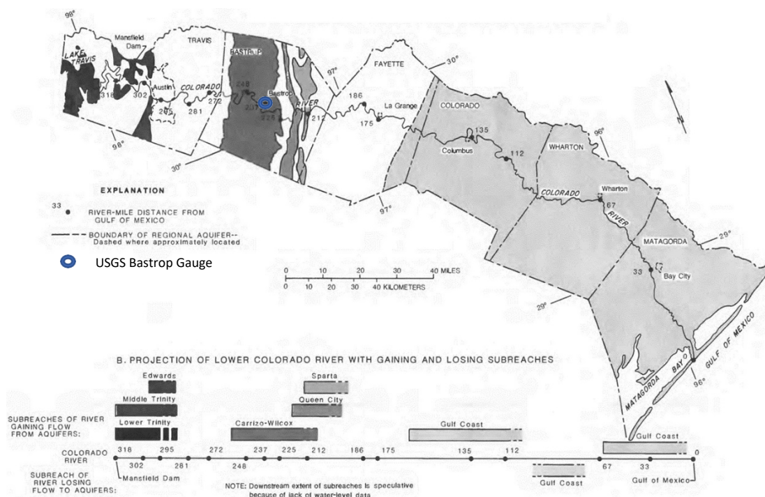
Figure 3. Location of gaining and losing stream reaches along the Colorado River based on contours of water level developed using data from 1970 to 1985 and from regional aquifers in the lower Colorado River Basin (from Woodward, 1989). From Young et al. 2017, Figure 4-12.
