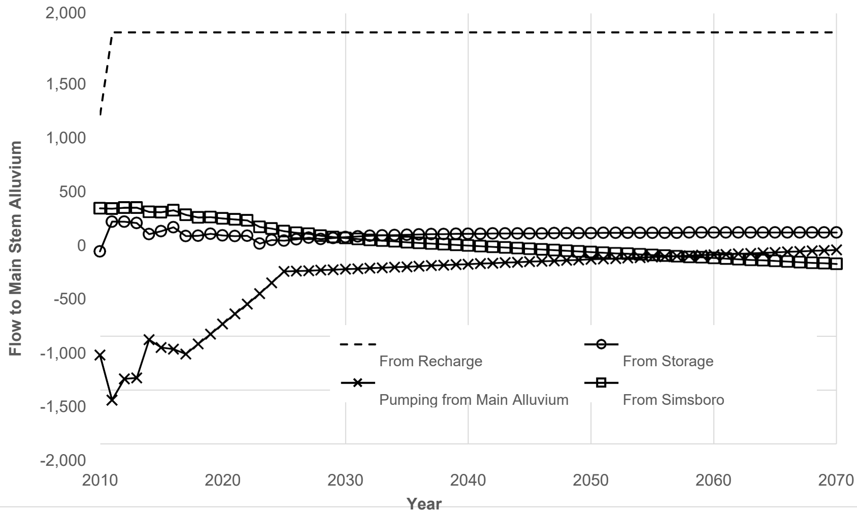
GAM Estimates of Flows to Alluvium Along Main Stem of the Colorado River (S-19) (b)
