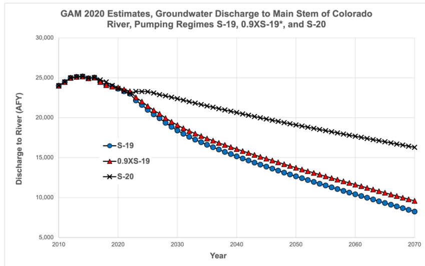
Figure 9. Effects of S-19 with 10% variance applied (0.9XS-19) compared to S-19 and S-20 Pumping on Groundwater Discharge to the Colorado River
