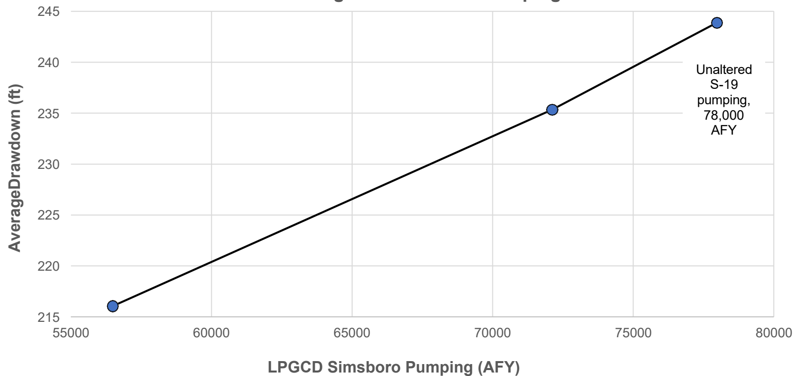
Figure 1 Effects of Varying S-19 Pumping on Average Simsboro Drawdowns in LPGCD
