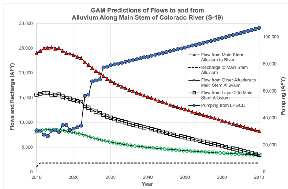
Figure 7. GAM predictions of flows to and from the Colorado River using S-19 pumping file (Figure 2 in The Rice Reports, Appendix 8).
