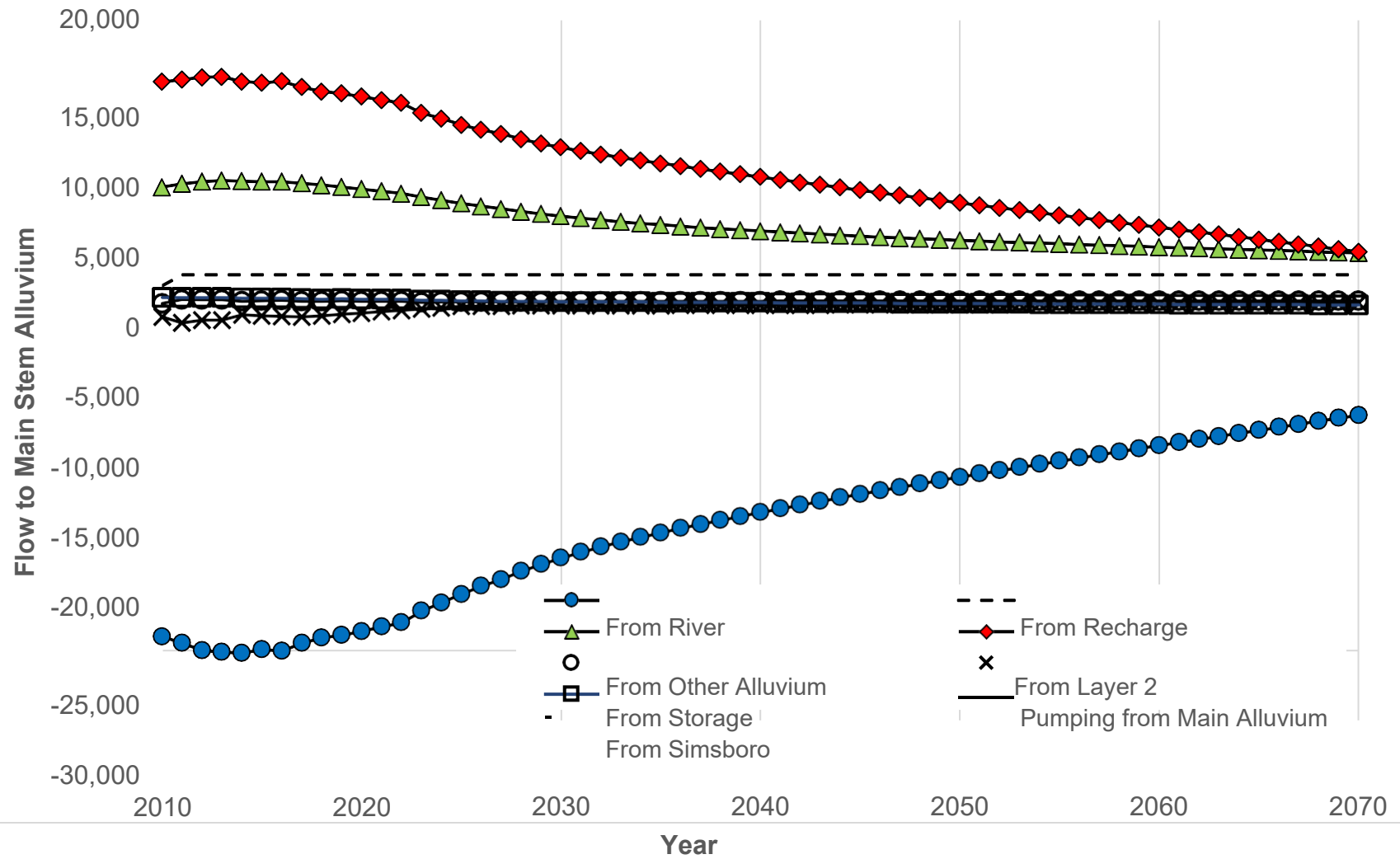
GAM Estimates of Flows to Alluvium Along Main Stem of the Colorado River (S-19) (a)
