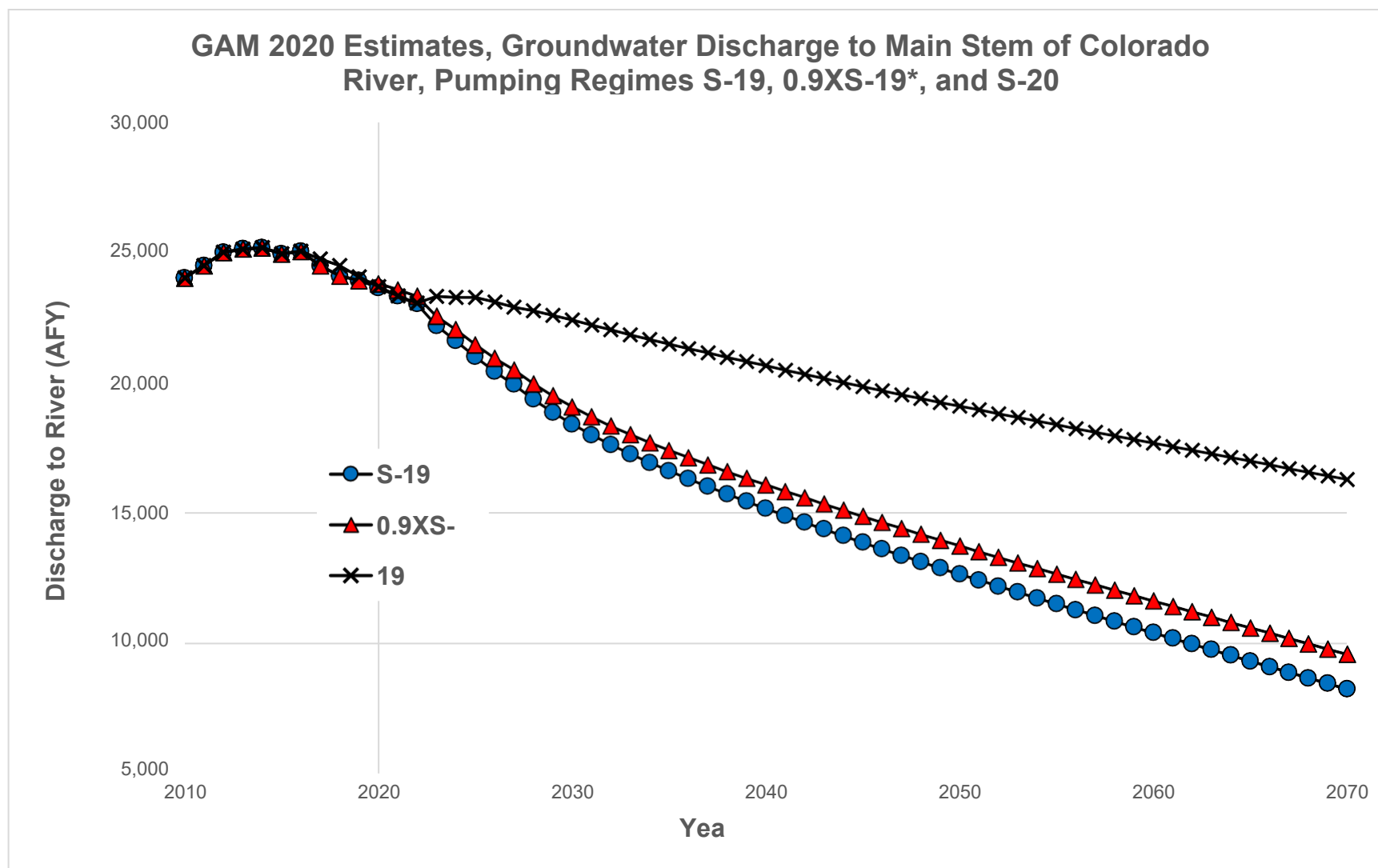
Figure 1 Effect of Pumping Regimes on Groundwater Discharge to Main Stem of Colorado River (*Pumping from the Simsboro and Carrizo aquifers in the LPGCD decreased by 10%)
