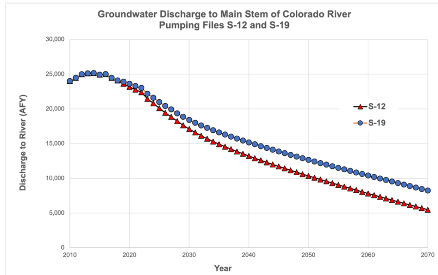
Figure 8. Effects of S-19 and S-12 Pumping on Groundwater Discharge to the Colorado River
