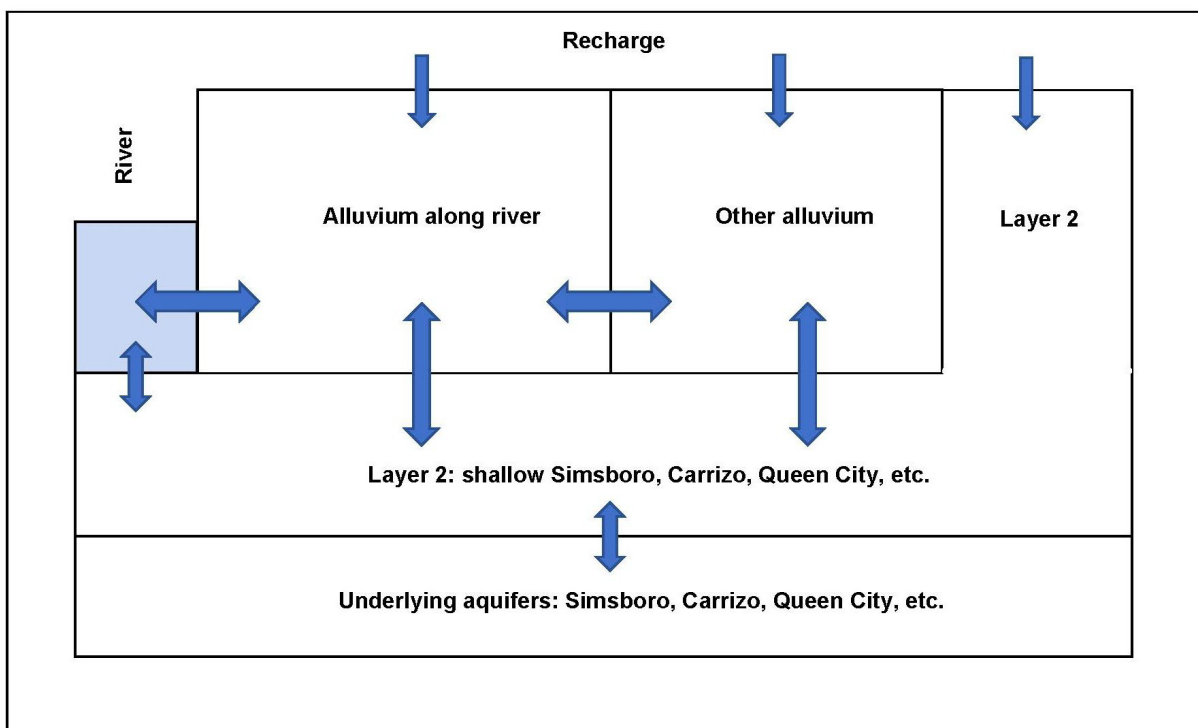
Figure 6. Schematic of flow relationships simulated by the GAM. (Figure 1 in Rice Report, Appendix 8)
