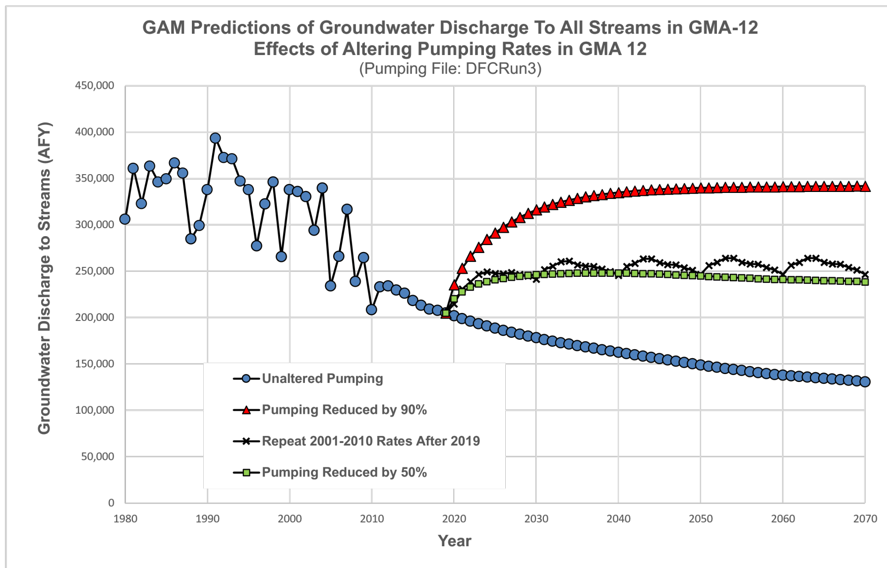
Figure A3-2 Pumping File DFCRun3, Effects of Reduced Pumping on Groundwater Discharge to All Streams in GMA-12
