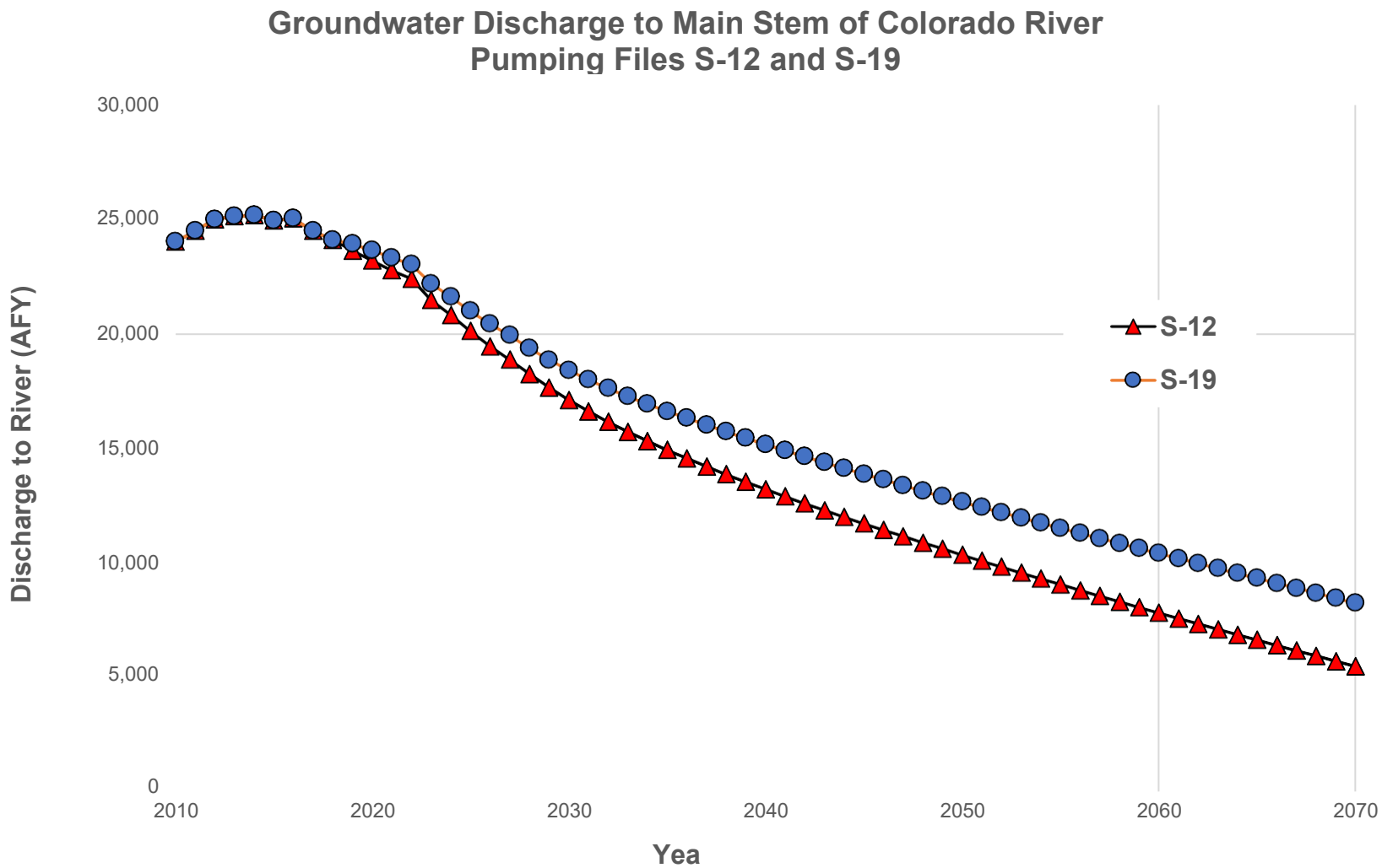
Figure 2 Effects of S-19 and S-12 Pumping on Groundwater Discharge to the Colorado River
